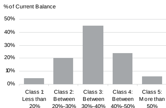
DTI Distribution
